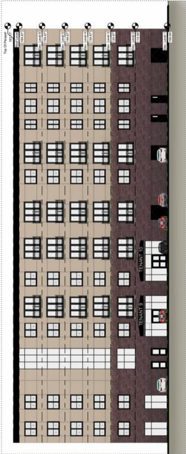
South Elevation
